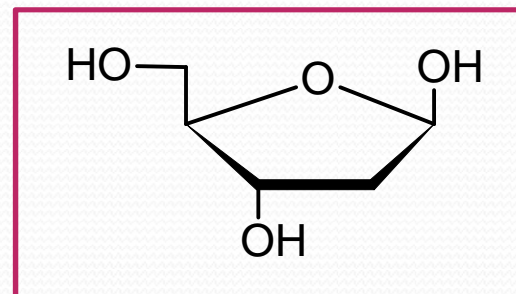
2'-deoxy- \beta -D-ribofuranosa
