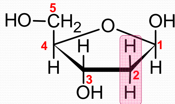
2'-deoxy- \beta -D-ribofuranosa
